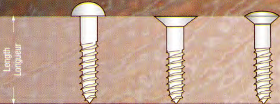
ROUND RONDE FLAT FRAISEE OVAL OVALE
