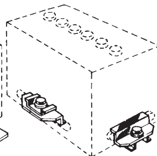
Card No. 570-510 Universal side type for side mount battery groups 22F and 24C also end mount group 22F.
