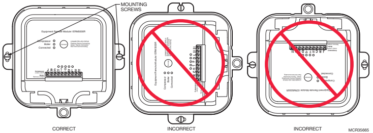
Fig. 11. Mounting orientation.
