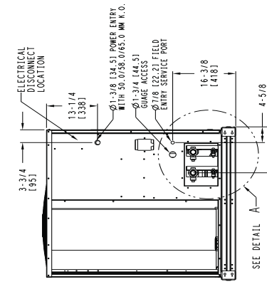
LEFT SIDE VIEW FOR 38AOLD SYSTEMS
