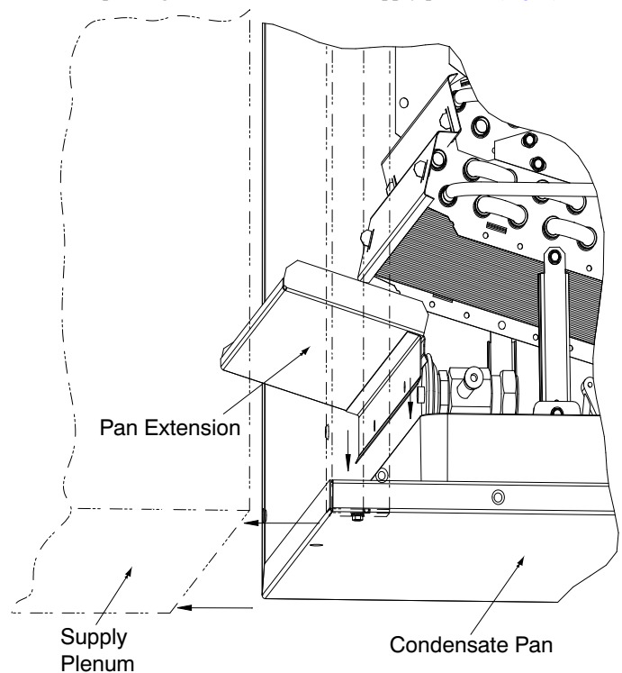
Fig. 2 – Horizontal-Left Installation of Pan Extension (43, 60 & 61 sizes only)
