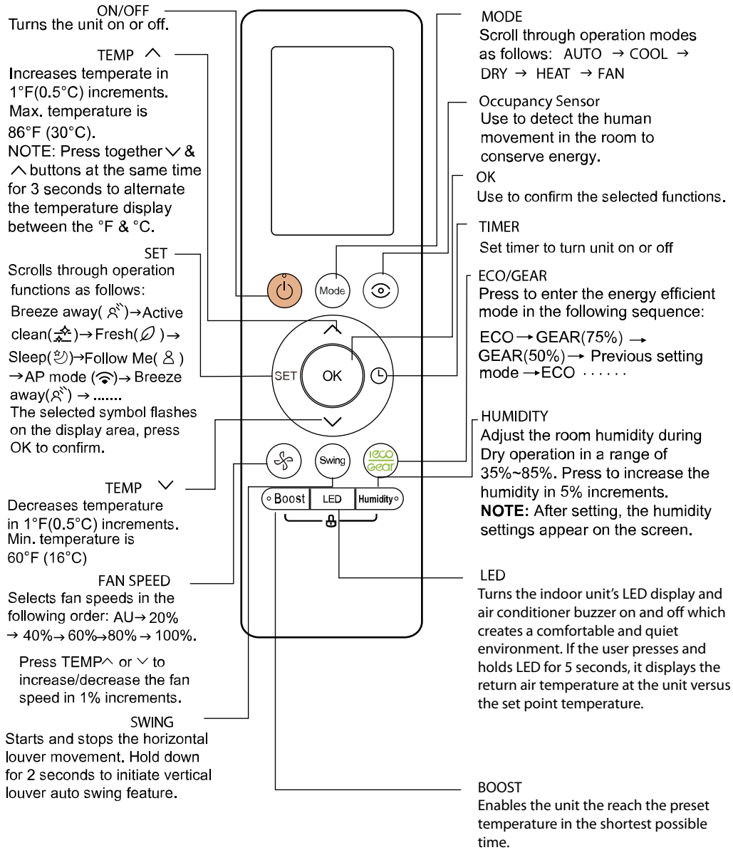
Fig. 2 —Remote Control Functions
